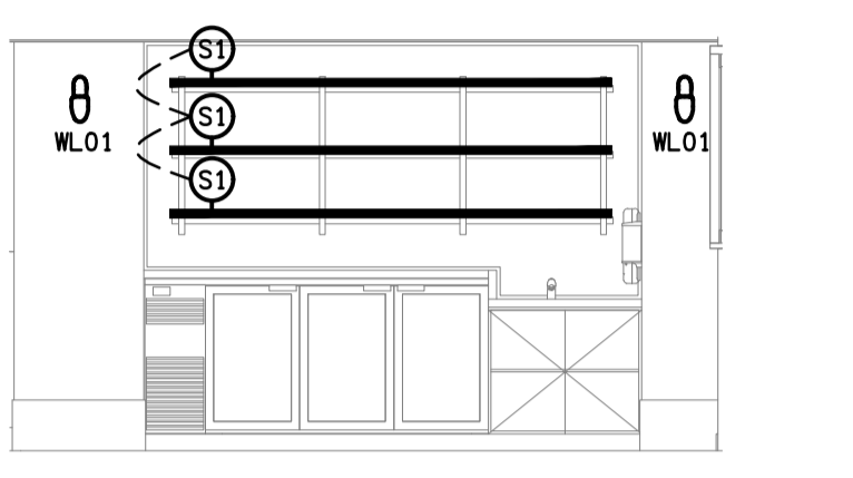
DETAIL 3 FUNCTION BAR REAR WALL ELEVATION SCALE 1: 50
