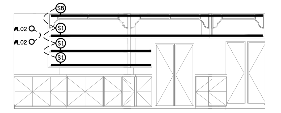
DETAIL 4 / 5 / 6 GAMING BAR REAR WALL ELEVATION SCALE 1: 50
